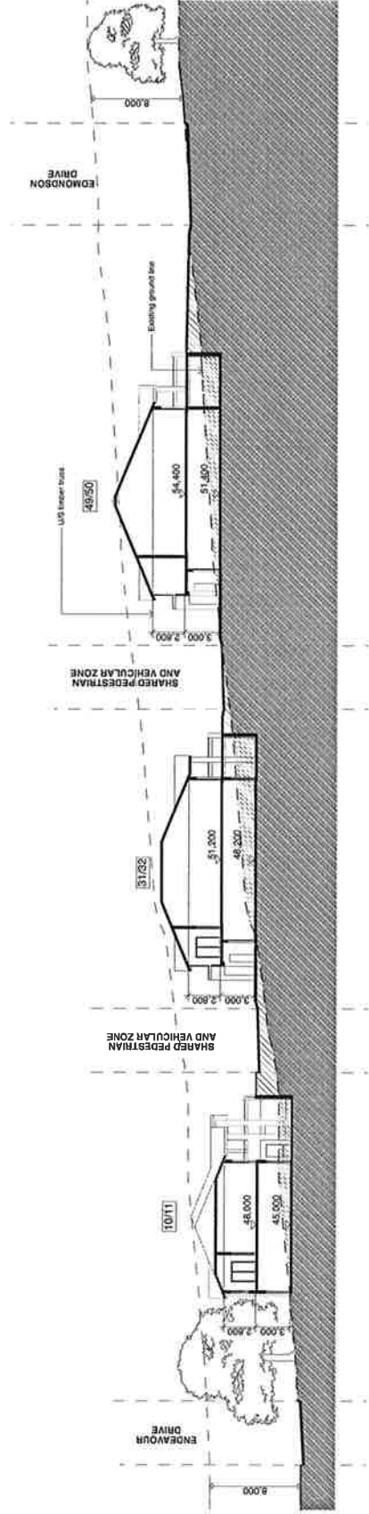
2 SECTION A 1:200
